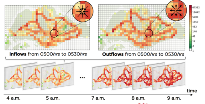
Figure 1. Visual representation of spatio-temporal crowd flows with a time series of 3D 2-channel images.
